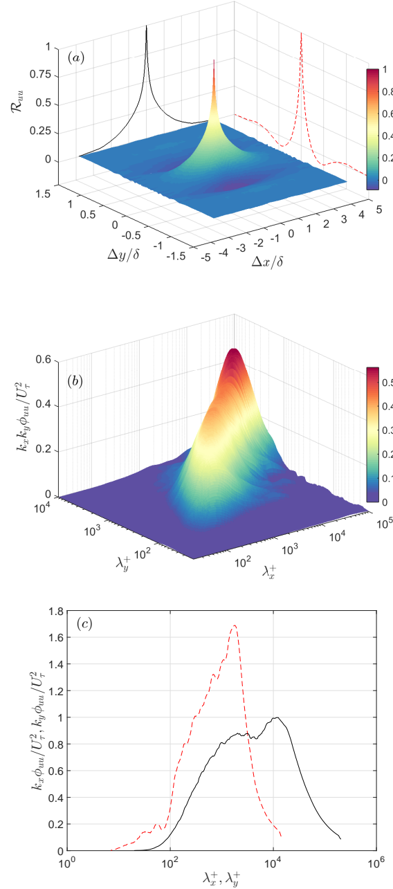
Figure 2: (a) Normalised 2-D correlation constructed from the velocity time series with projections of 1-D correlations at \Delta x = 0 and \Delta y = 0 , (b) 2-D spectra obtained from the 2-D correlation and (c) 1-D streamwise (—) and 1-D spanwise (- - -) spectra obtained by integrating the 2-D spectra.
