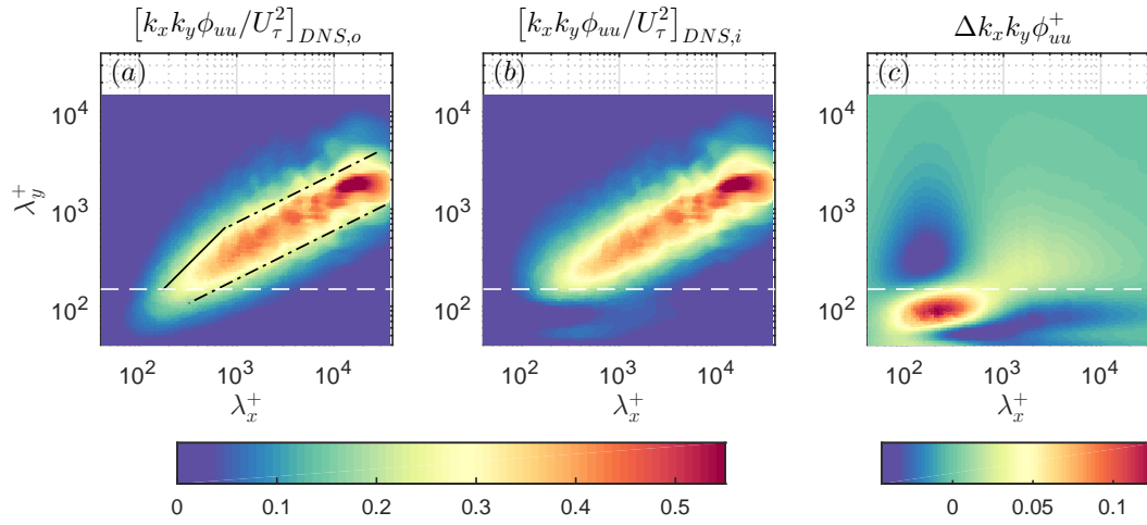
Figure 5: (a) 2-D spectra obtained from the original DNS correlation, where — and - - - represent the relationships \lambda_y/z \sim \lambda_x/z and \lambda_y/z \sim (\lambda_x/z)^{1/2} respectively as reported by Del Alamo et al. [3], (b) 2-D spectra obtained from the interpolated DNS correlation and (c) difference between (a) and (b).
