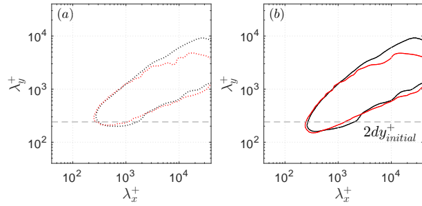
Figure 6: Comparison of experimental ( Re_\tau = 3350 ) and DNS ( Re_\tau \approx 2000 ) results at k_x k_y \phi_{uu} / U_\tau^2 = 0.15 , (a) before correction where, \cdots uncorrected experiment and \cdots interpolated DNS and (b) after correction where, — corrected experiment and — original DNS
