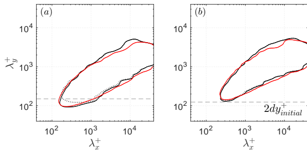
Figure 3: Comparison of experimental and DNS results for k_x k_y \phi_{uu} / U_\tau^2 = 0.15 at Re_\tau \approx 2000 and, (a) z^+ \approx 100 and (b) z^+ \approx 200 ; where, \cdots uncorrected experiment; \text{---} corrected experiment and \text{---} DNS
