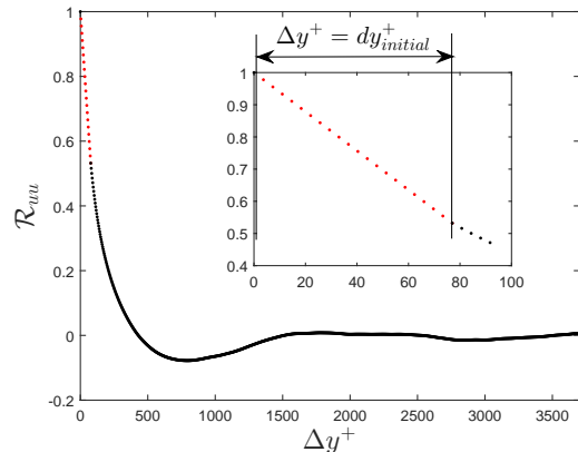
Figure 4: 1-D spanwise correlation demonstrating the method of correcting dy_{initial}^+ error.
